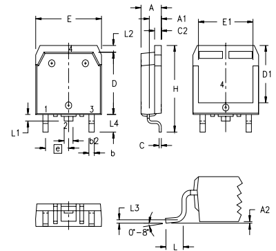
TO-268 (IXFT) Outline
