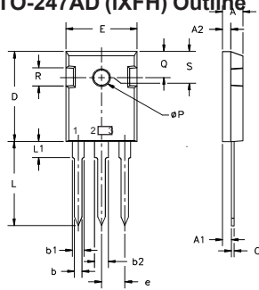
TO-247AD (IXFH) Outline
