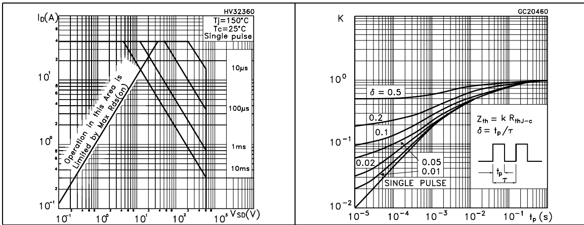
Figure 6. Safe operating area for DPAK, IPAK
