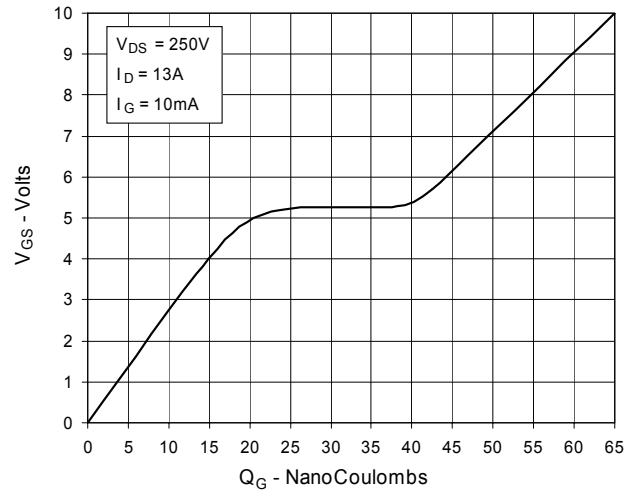
Fig. 10. Gate Charge
