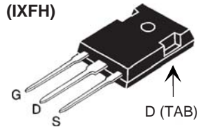
TO-3P (IXFQ)
