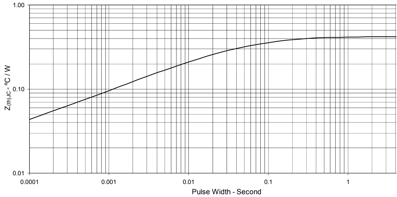
Fig. 19. Maximum Transient Thermal Impedance
