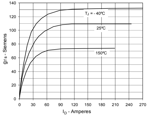
Fig. 8. Transconductance
