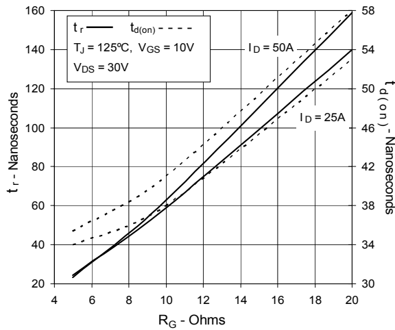
Fig. 15. Resistive Turn-on Switching Times vs. Gate Resistance
