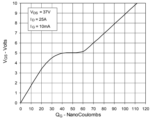
Fig. 10. Gate Charge
