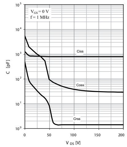
Fig. 9 Typ. capacitances
