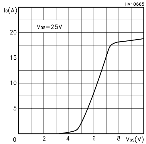
Transfer Characteristics
