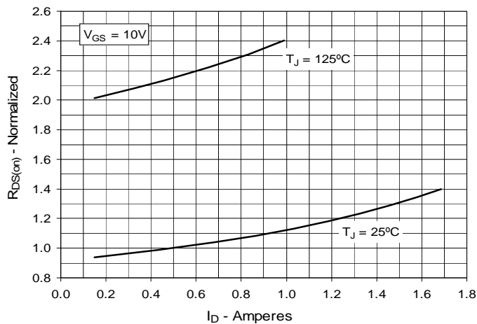
Fig. 5. R_{DS(on)} Normalized to I_D = 0.5A Value vs. Drain Current
