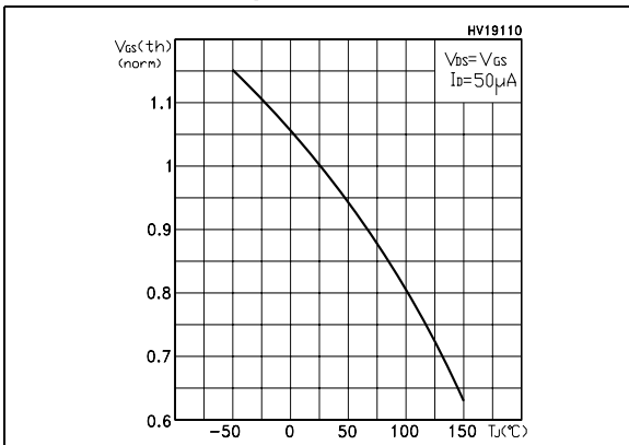
Figure 12. Normalized gate threshold vs temperature
