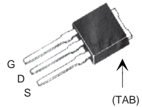
TO-252 (IXTY)
