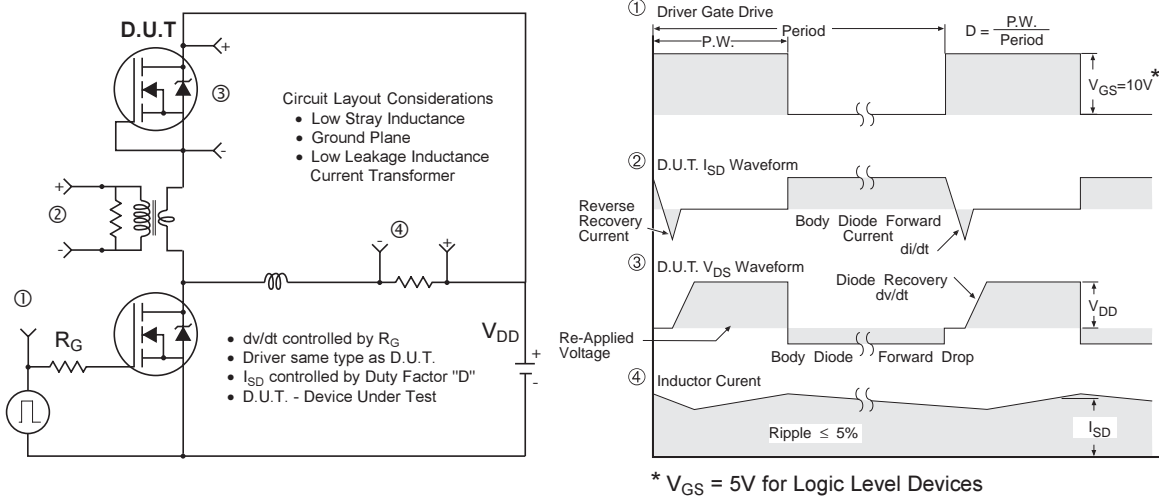
Fig 15. Peak Diode Recovery \frac{dv}{dt} Test Circuit for N-Channel HEXFET ® Power MOSFETs
