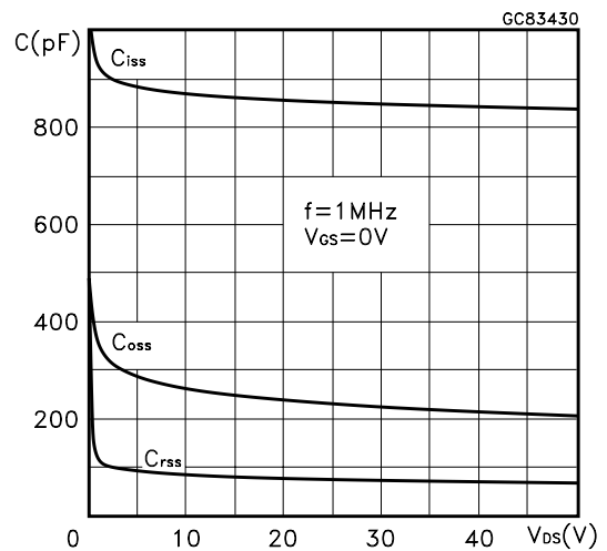
Capacitance Variations
