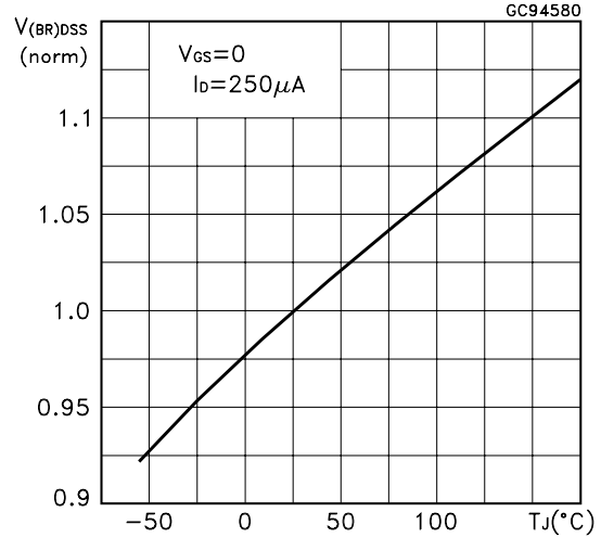
Normalized Breakdown Voltage Temperature
