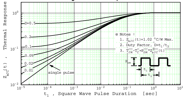
Fig 11. Thermal Response
