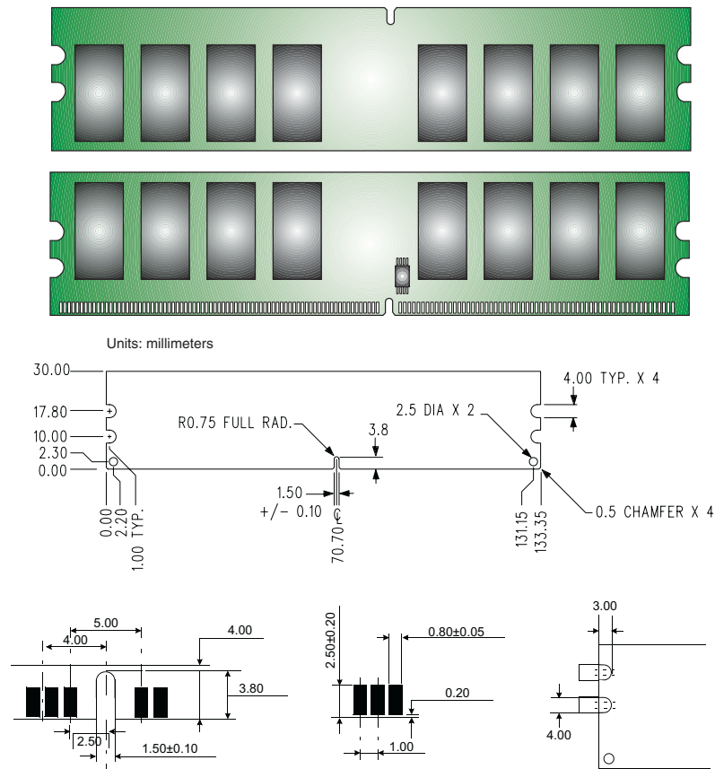
Figure 1: KVR800D2N5/2G 240-Pin DIMM
