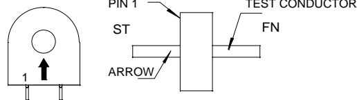
POLARITY DETAIL TOP VIEW
