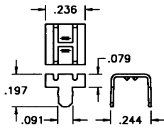
Mounting Detail For Two Clips
