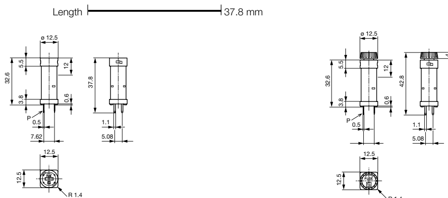
Variant Fingergrip 3101.0045
