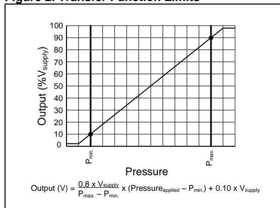
Figure 2. Transfer Function Limits
