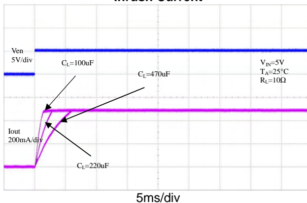
Inrush Current
