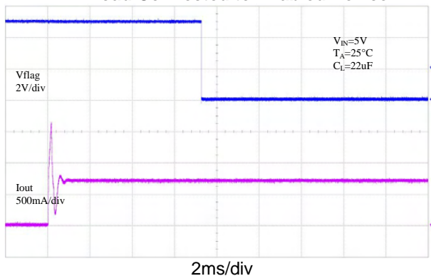
2 Ω Load Connected to Enabled Device
