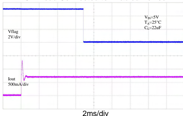
3 Ω Load Connected to Enabled Device
