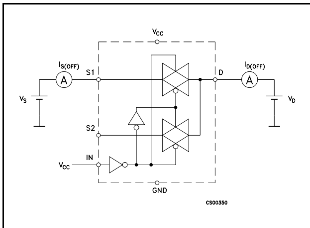
Figure 5: Off Leakage
