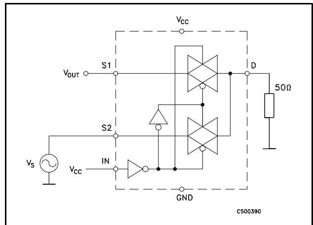
Figure 8: Channel To Channel Crosstalk
