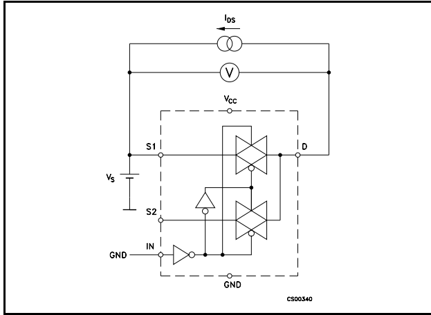
Figure 4: On Leakage
