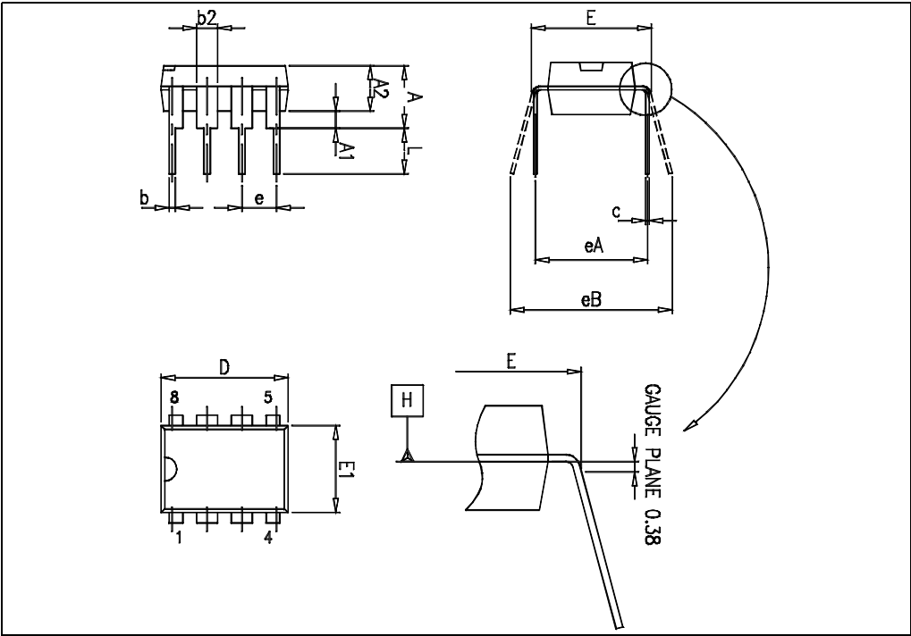
Figure 15. Package Dimensions
