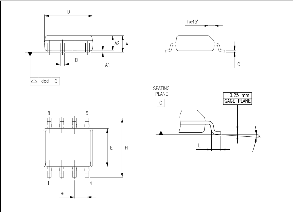
Figure 16. Package Dimensions
