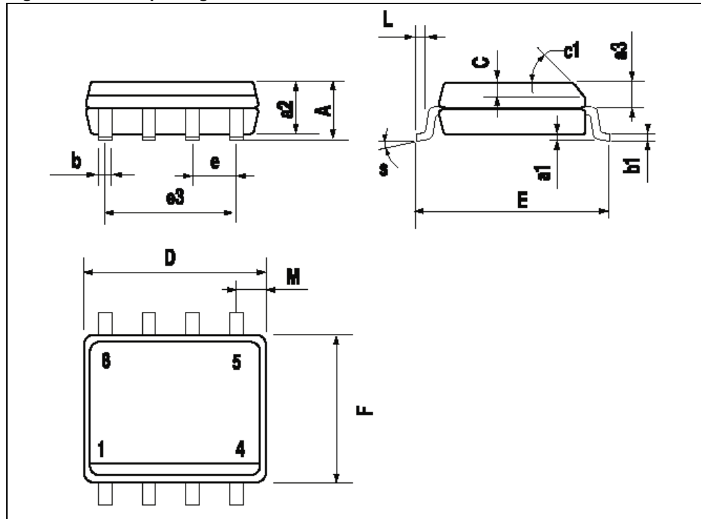
Figure 40. SO-8 package dimensions
