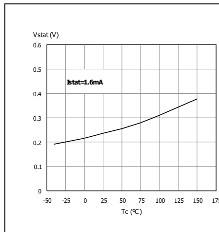
Figure 11. Status low output voltage
