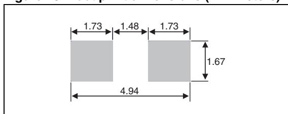
Figure 13: Foot print dimensions (millimeters)
