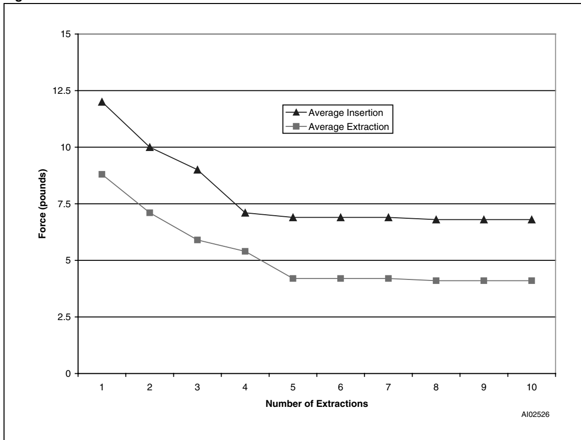
Figure 2. SNAPHAT ® insertion/extraction forces
