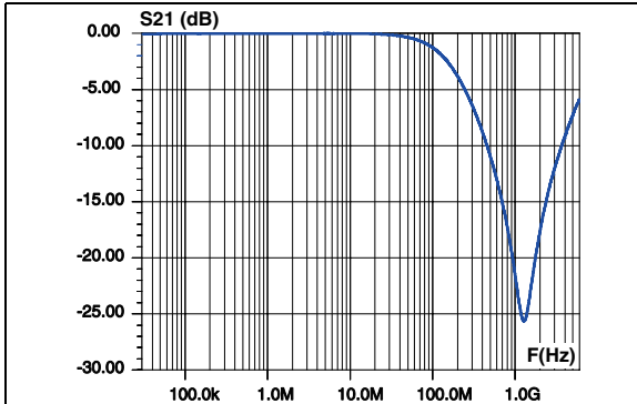
Figure 9. S21 attenuation measurement results of each channel
