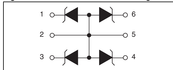
Figure 2. ESDAxxSC6 functional diagram
