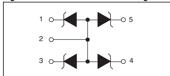
Figure 1. ESDAxxSC5 functional diagram
