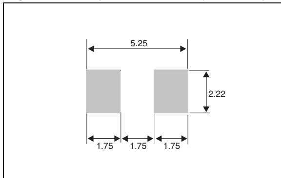
Figure 9. Footprint dimensions (millimeter)
