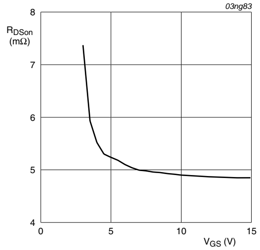
Fig 6. Drain-source on-state resistance as a function of gate-source voltages; typical values
