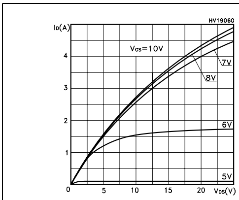
Figure 5. Output characteristics
