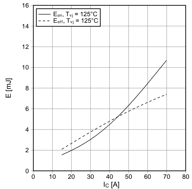
Schaltverluste IGBT-Wechselr. (typisch) switching losses IGBT-inverter (typical) E_{on} = f(I_c) , E_{off} = f(I_c) V_{GE} = \pm 15\text{ V} , R_{Gon} = 13\ \Omega , R_{Goff} = 13\ \Omega , V_{CE} = 600\text{ V}
