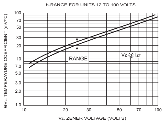
FIG.7- TEMPERATURE COEFFICIENTS
