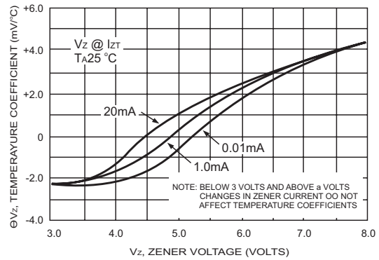
FIG.8- EFFECT OF ZENER CURRENT
