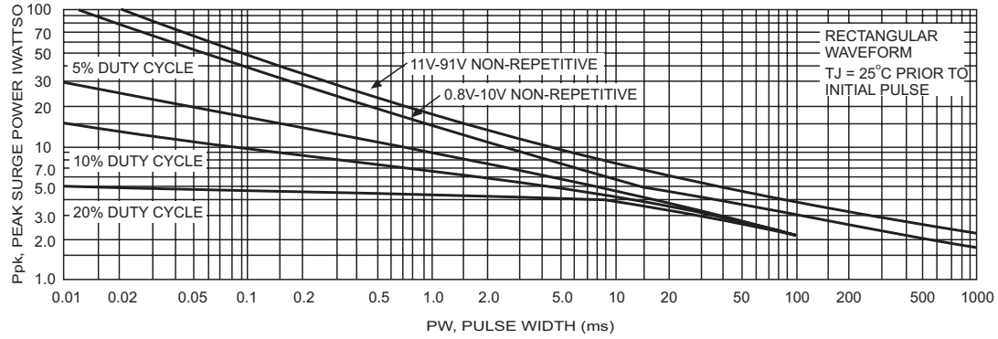
FIG.10- MAXIMUM SURGE POWER
