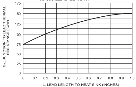
FIG.9- TYPICAL THERMAL RESISTANCE versus LEAD LENGTH
