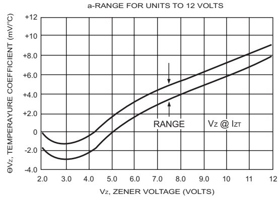
FIG.7- TEMPERATURE COEFFICIENTS
