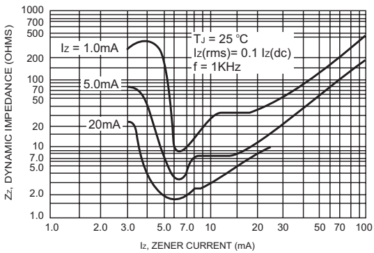
FIG.4- EFFECT OF ZENER VOLTAGE ON ZENER IMPEDANCE
