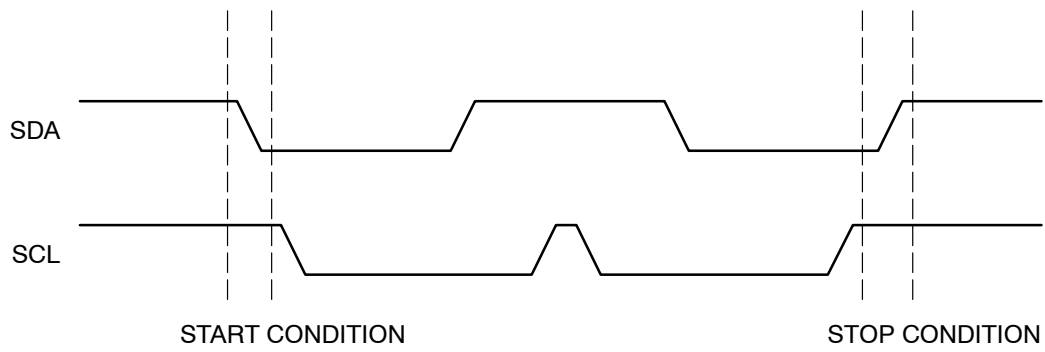
Figure 19. Start/Stop Condition
