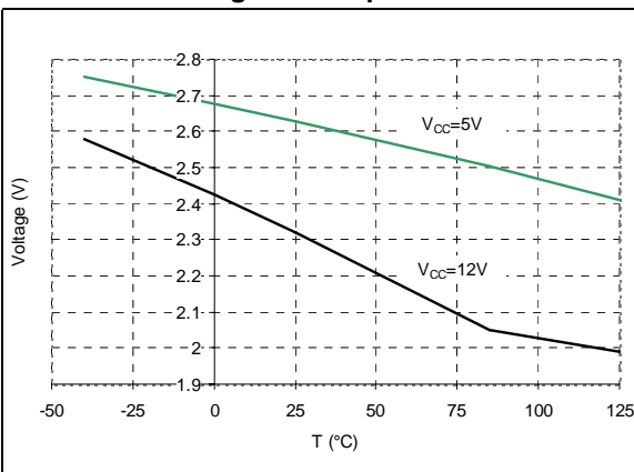
Figure 6. Minimum common mode operating voltage vs. temperature
