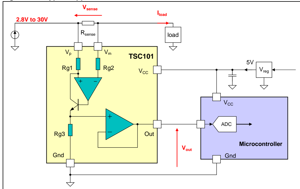
Figure 23. Typical application schematic
