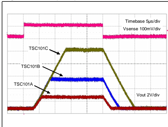
Figure 19. Step response
