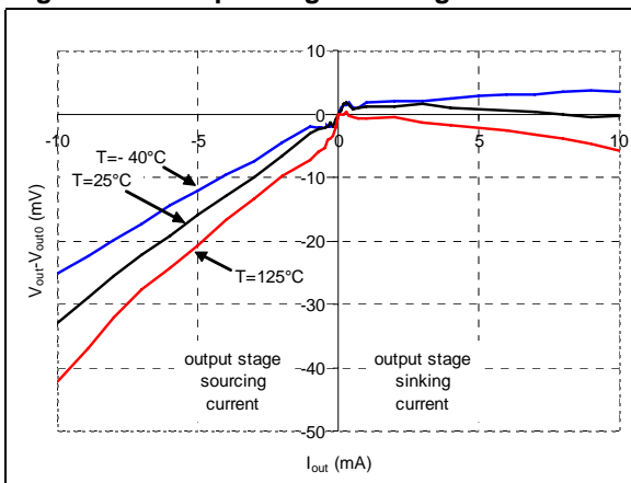
Figure 11. Output stage load regulation
