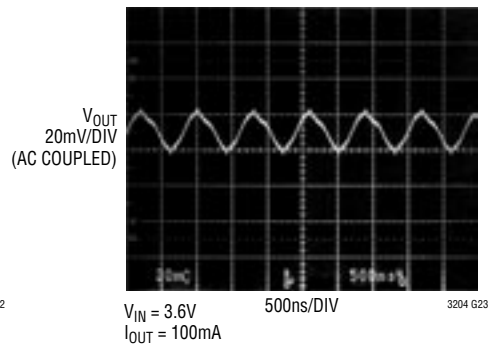
Output Ripple
