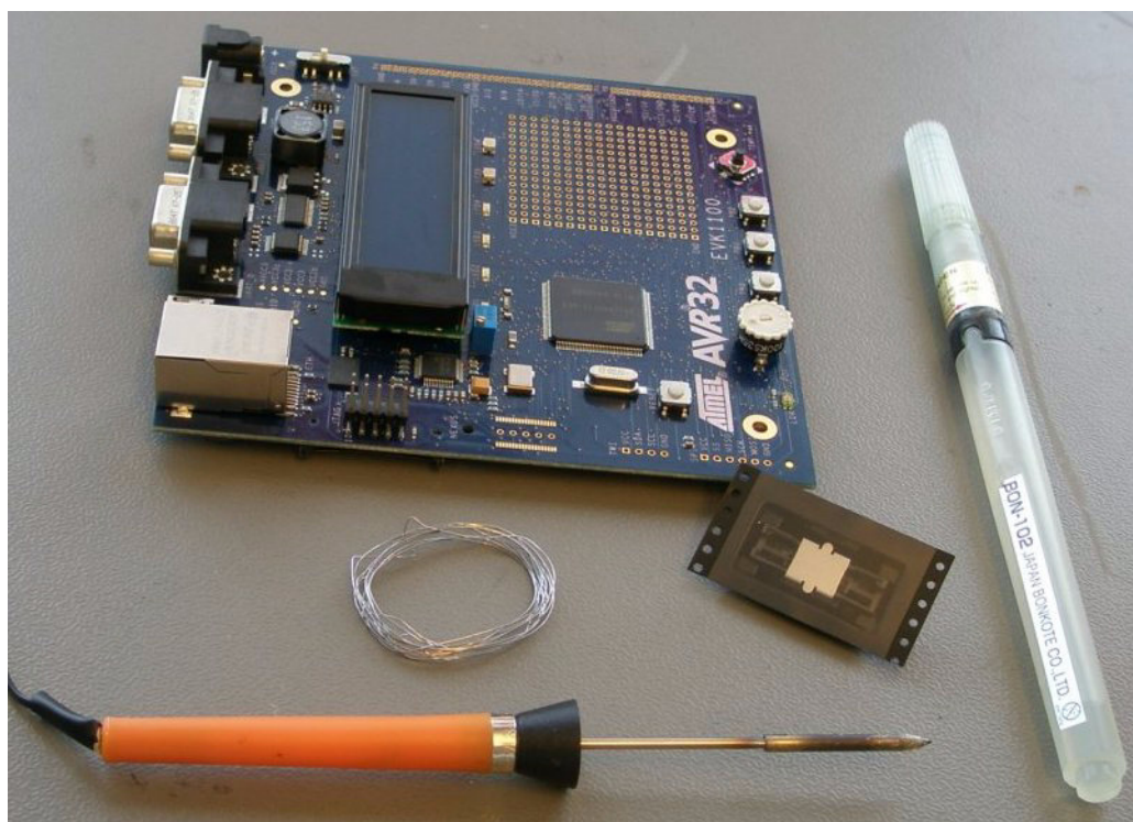
Figure 3-1. Required hardware and tools for installation of Mictor38
