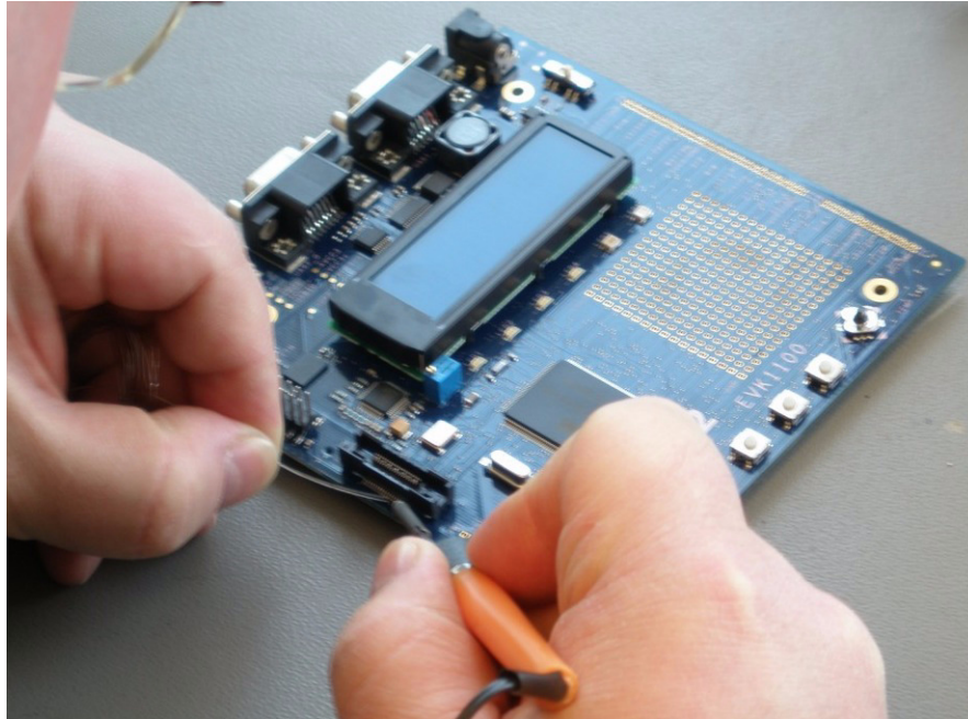
Figure 3-4. Soldering the corners
