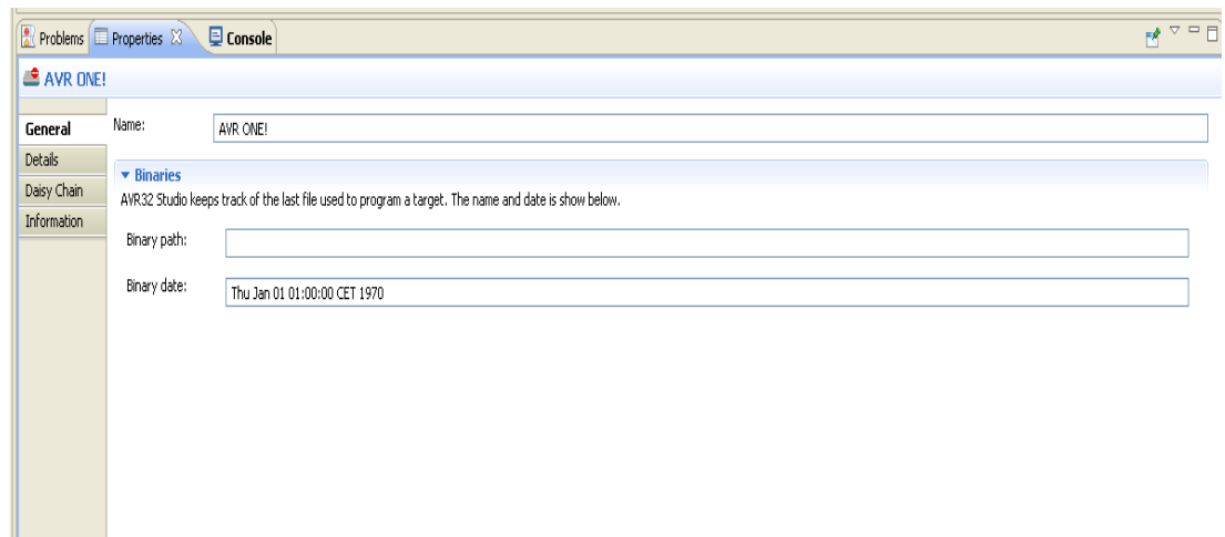
Figure 6-8. Properties view
