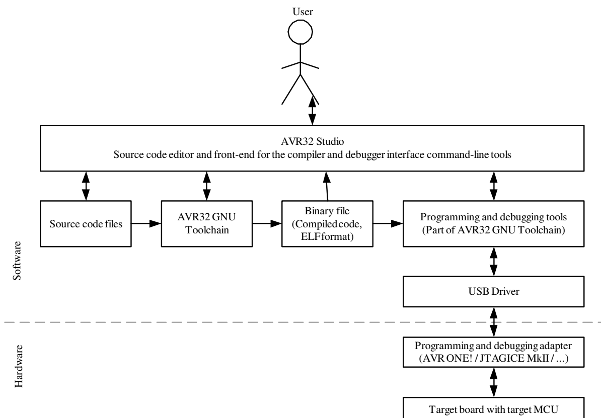
Figure 4-1. Tools structure
