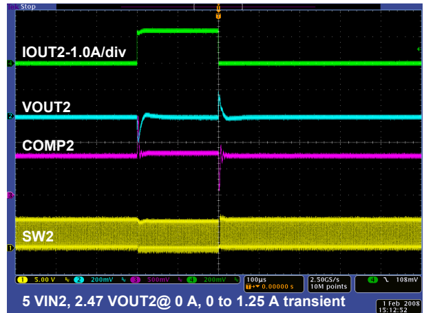
Figure 16. CH2 Transient Response
