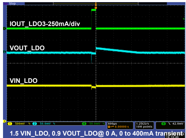
Figure 18. LDO Transient Response
