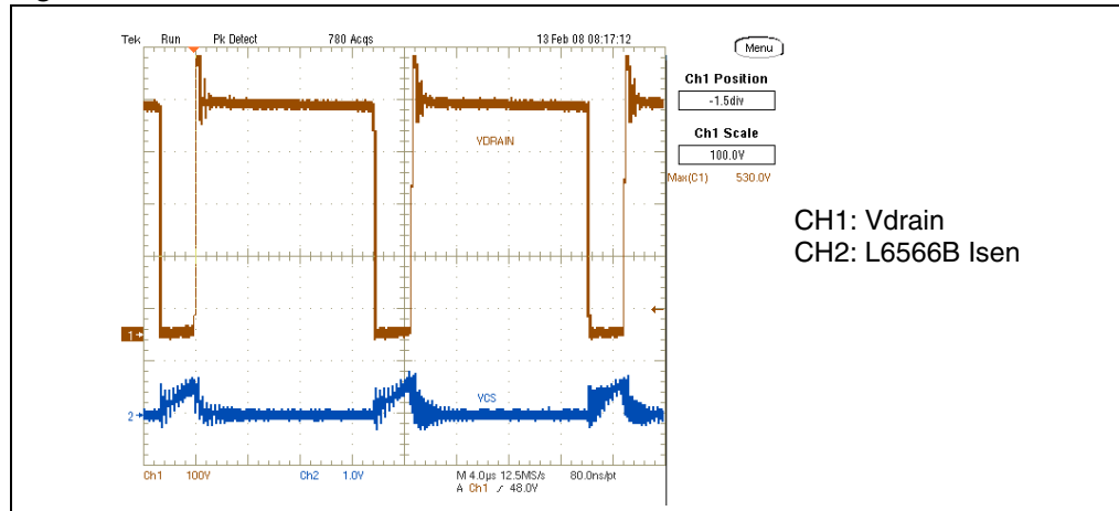
Figure 5. EVL6566B-40WSTB waveforms at 265 V-50 Hz - full load
