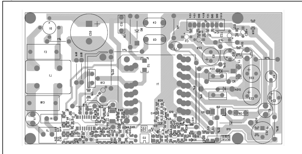
Figure 37. Silk screen - bottom side
