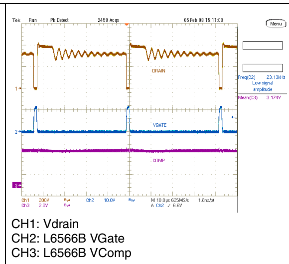
Figure 7. EVL6566B-40WSTB waveforms at 230 V - Pin=4 W
