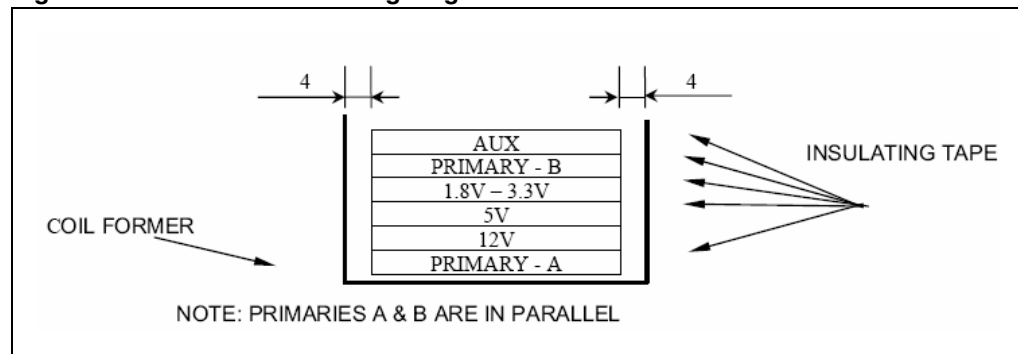
Figure 39. Transformer winding diagram
