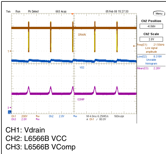
Figure 8. EVL6566B-40WSTB waveforms at 265 Vac - no load
