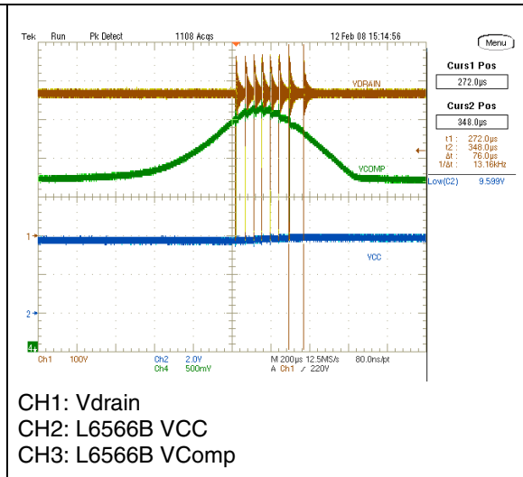
Figure 9. EVL6566B-40WSTB waveforms at 265 Vac - no load (detail)
