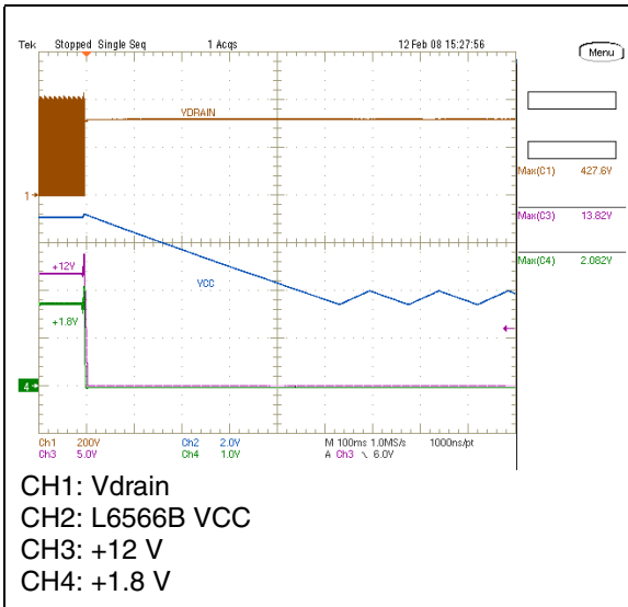
Figure 30. EVL6566B-40WSTB OVP at 230 Vac- full load
