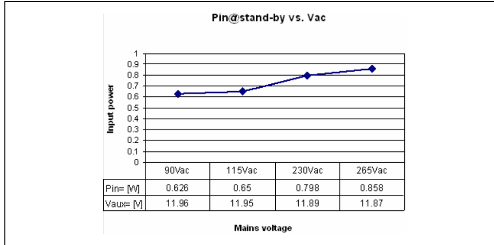
Figure 10. Input power vs. mains voltage during standby
