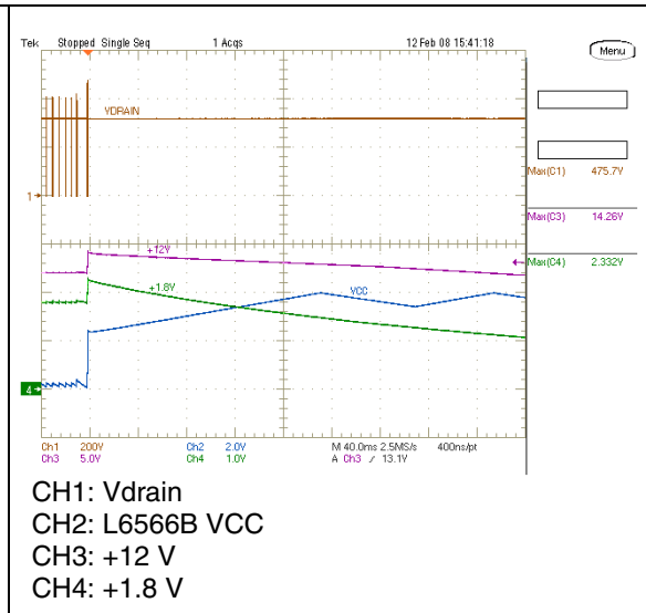
Figure 31. EVL6566B-40WSTB OVP at 230 Vac- no load
