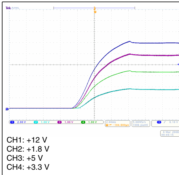
Figure 14. EVL6566B-40WSTB startup at 90 Vac - full load
