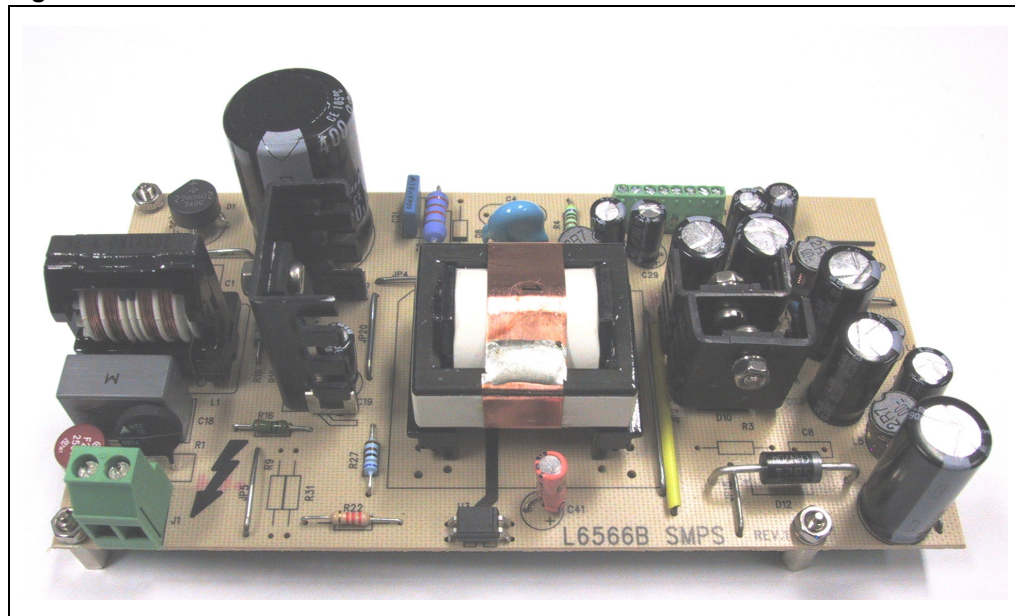
Figure 1. EVL6566B-40WSTB demonstration board
