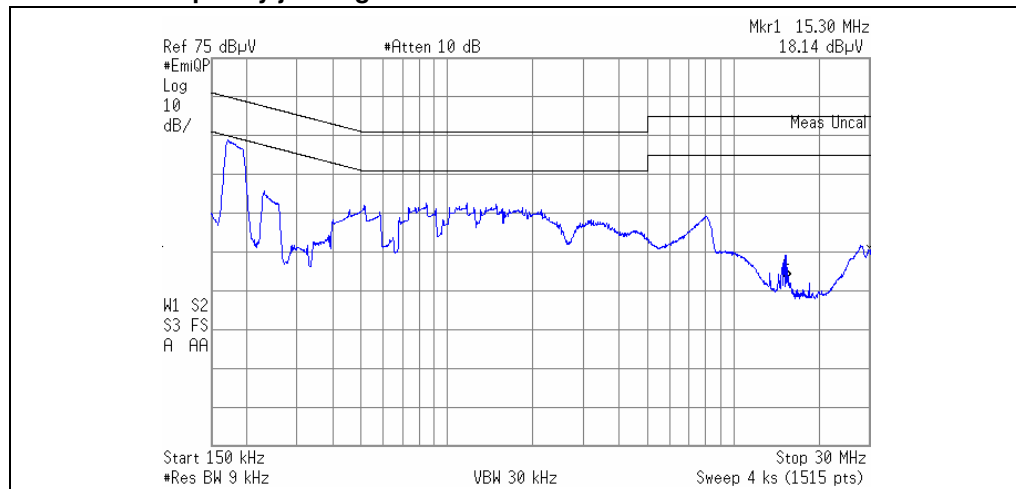
Figure 33. EVL6566B-40WSTB conducted noise measurement phase A with frequency jittering
