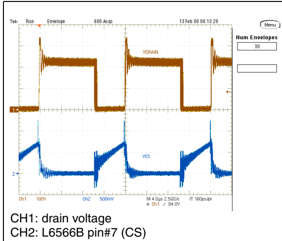
Figure 3. EVL6566B-40WSTB waveforms at 115 Vac-60 Hz - full load
