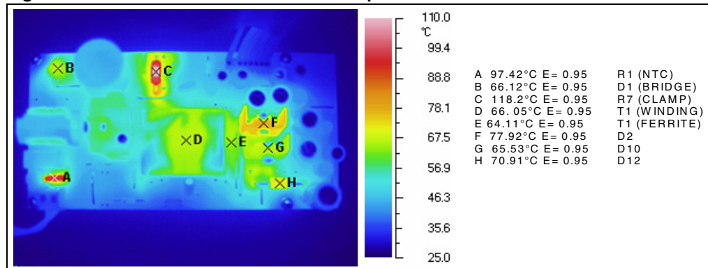
Figure 34. EVL6566B-40WSTB thermal map at 115 Vac - full load
