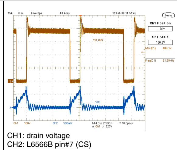
Figure 4. EVL6566B-40WSTB waveforms at 230 Vac-50 Hz - full load
