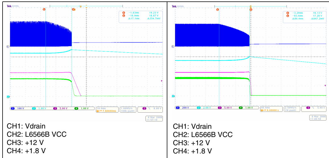
Figure 16. EVL6566B-40WSTB hold-up time at 115 Vac - full load Figure 17. EVL6566B-40WSTB hold-up time at 230 Vac - full load
