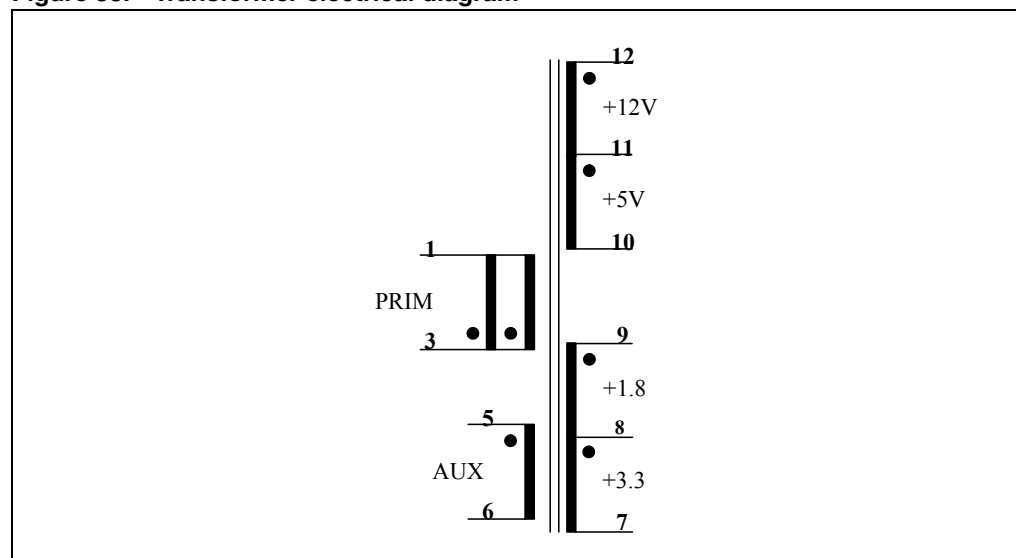
Figure 38. Transformer electrical diagram
