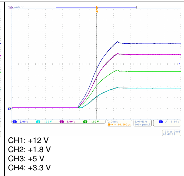
Figure 15. EVL6566B-40WSTB startup at 265 Vac - full load
