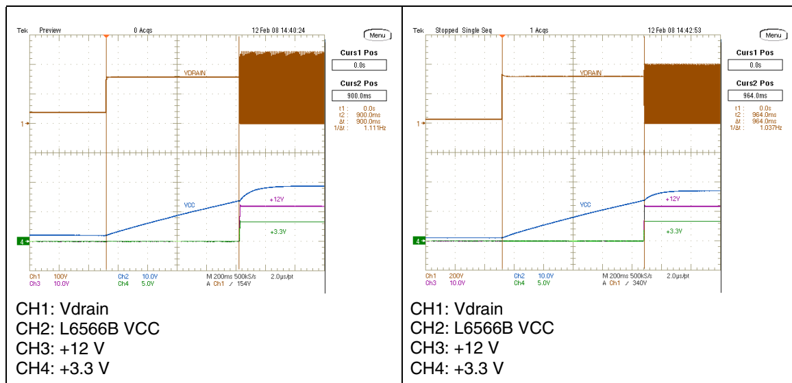
Figure 12. EVL6566B-40WSTB wakeup time at 115 Vac Figure 13. EVL6566B-40WSTB wakeup time at 230 Vac
