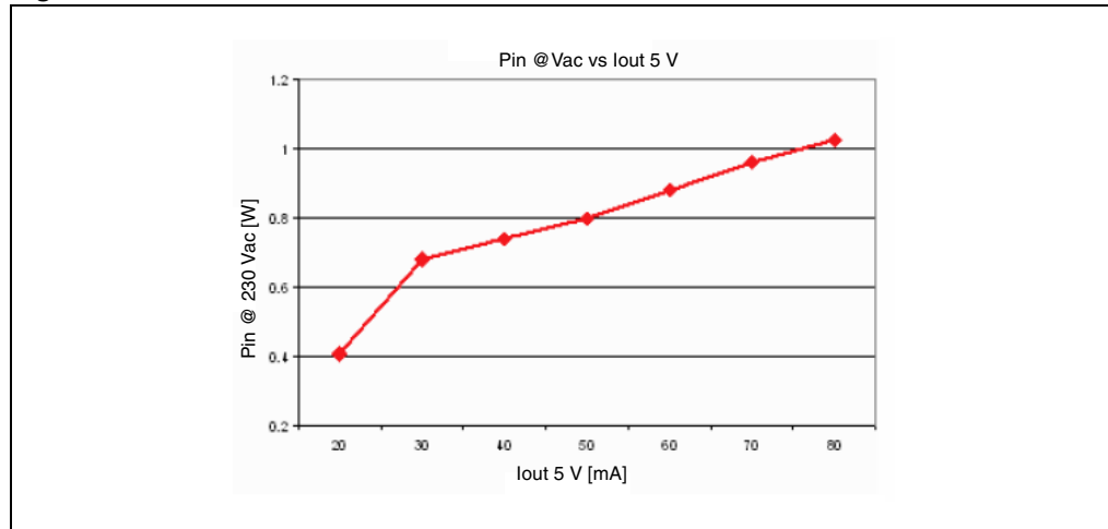
Figure 11. Pin at 230 Vac vs. Iout 5 V
