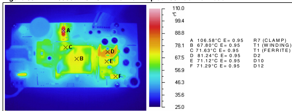
Figure 35. EVL6566B-40WSTB thermal map at 230 Vac - full load
