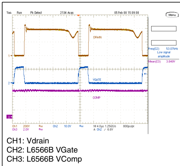
Figure 6. EVL6566B-40WSTB waveforms at 230 V - Pin=30 W
