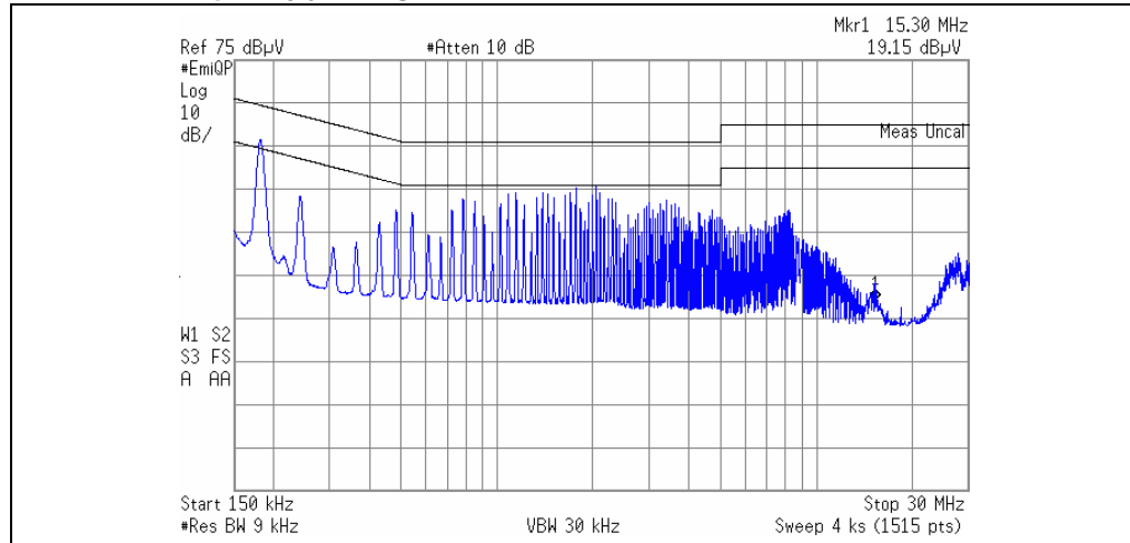
Figure 32. EVL6566B-40WSTB conducted noise measurement phase A without frequency jittering
