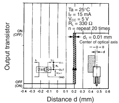
Repeat Sensing Position Characteristics (Typical)
