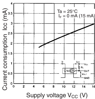
Current Consumption vs. Supply Voltage (Typical)
