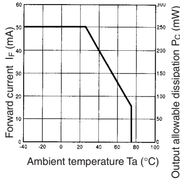
LED Current vs. Ambient Temperature Characteristics (Typical)
