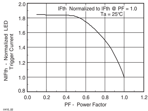
Figure 2. Normalized LED Trigger Current vs. Power Factor
