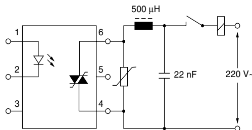
Figure 15. 3 - Connect a Choke of Low Winding Cap. in Series, e.g., a Ringcore Choke, with Higher Load Currents
