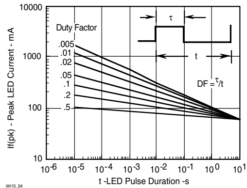
Figure 4. Peak LED Current vs. Duty Factor, Tau
