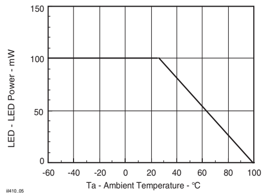
Figure 5. Maximum LED Power Dissipation
