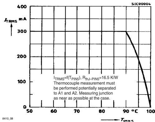
Figure 8. Current Reduction
