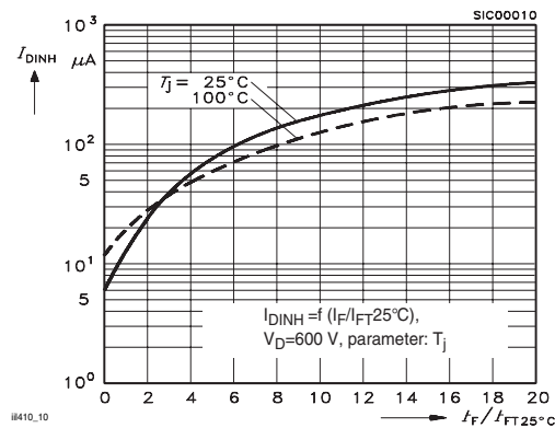
Figure 10. Typical Inhibit Current
