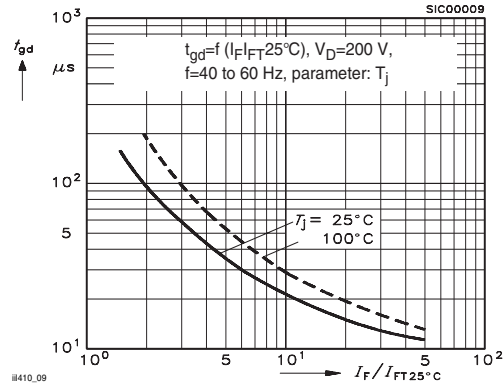
Figure 9. Typical Trigger Delay Time
