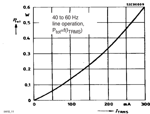
Figure 11. Power Dissipation 40 to 60 Hz Line Operation
