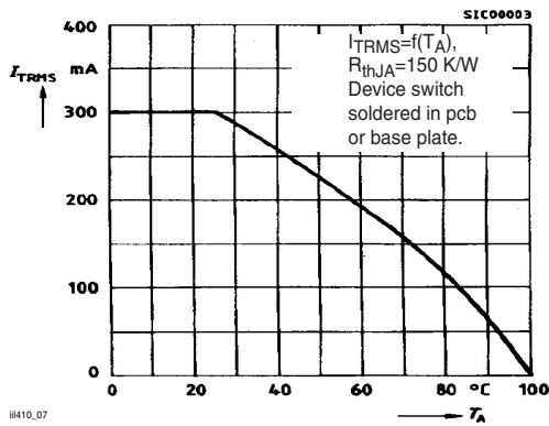
Figure 7. Current Reduction
