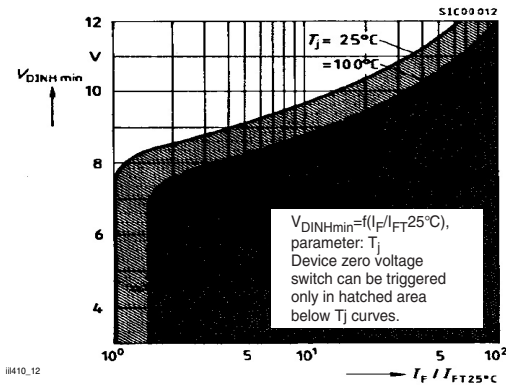
Figure 12. Typical Static Inhibit Voltage Limit
