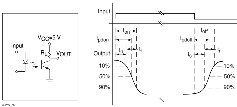
Figure 8. Switching Test Circuit
