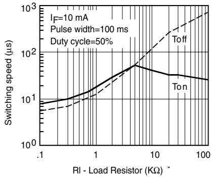
Figure 5. Switching Speed vs. Load Resistor
