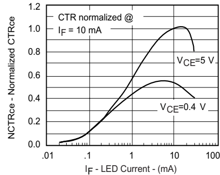
Figure 3. Normalized CTR_{ce} vs. Forward Current
