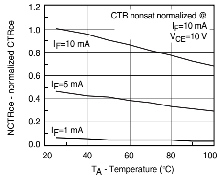
Figure 4. Current Transfer Ratio (normalized) vs. Ambient Temperature
