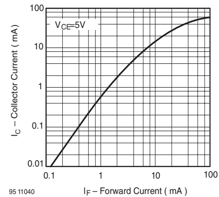
Figure 8. Collector Current vs. Forward Current
