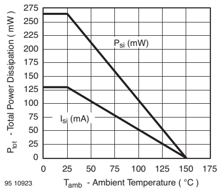
Figure 1. Derating diagram
