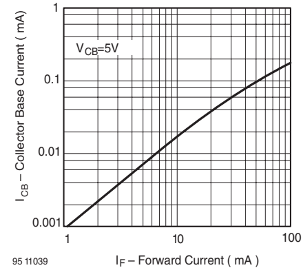
Figure 7. Collector Base Current vs. Forward Current
