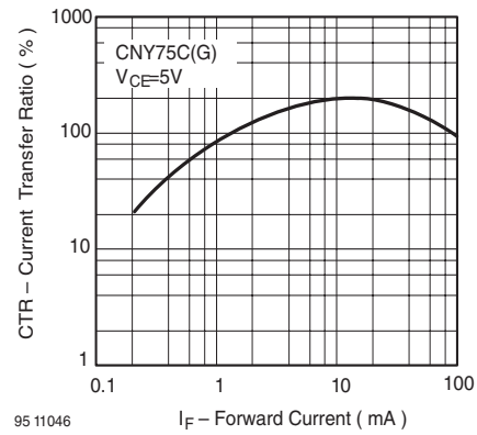
Figure 18. Current Transfer Ratio vs. Forward Current
