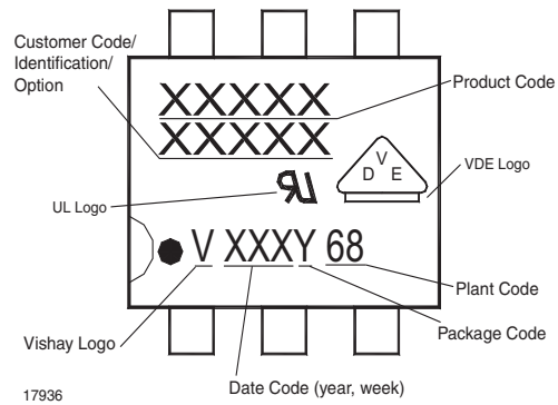
Figure 25. Marking example
