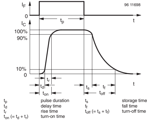
Figure 3. Switching Times
