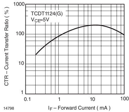
14798 Figure 13. Current Transfer Ratio vs. Forward Current
