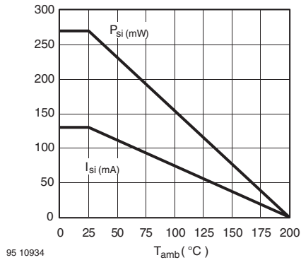
Figure 1. Derating diagram
