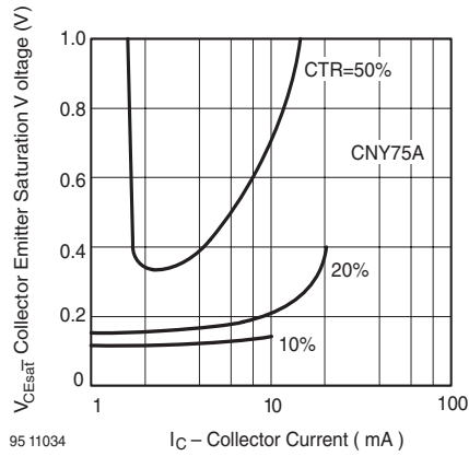
95 11034 Figure 10. Collector Emitter Saturation Voltage vs. Collector Current
