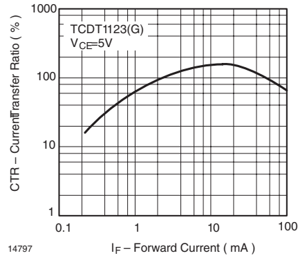
14797 Figure 12. Current Transfer Ratio vs. Forward Current
