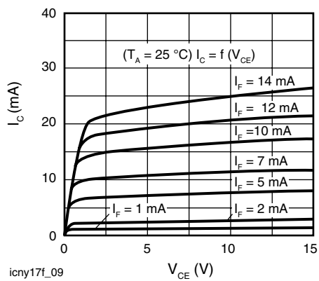
Fig. 9 - Output Characteristics CNY17F-2, -3
