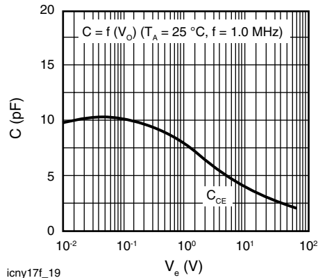
Fig. 19 - Transistor Capacitance
