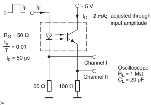
Figure 3. Test circuit, non-saturated operation
