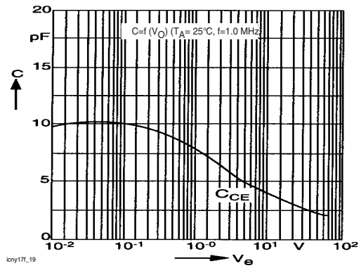
Figure 19. Transistor Capacitance
