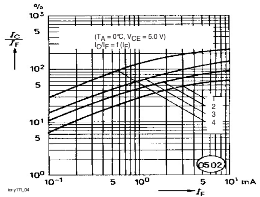
Figure 4. Current Transfer Ratio vs. Diode Current
