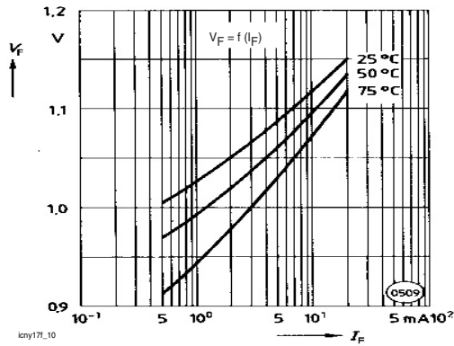
Figure 10. Forward Voltage
