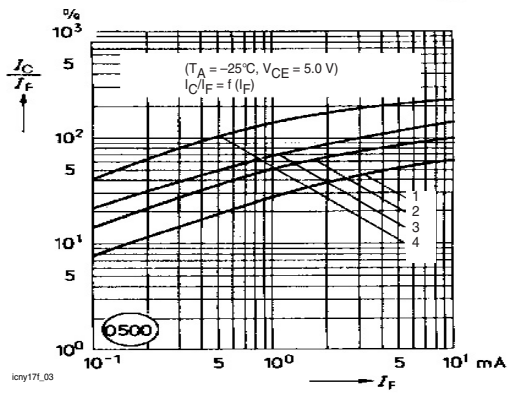
Figure 3. Current Transfer Ratio vs. Diode Current
