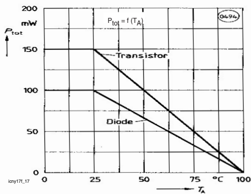
Figure 17. Permissible Power Dissipation for Transistor and Diode
