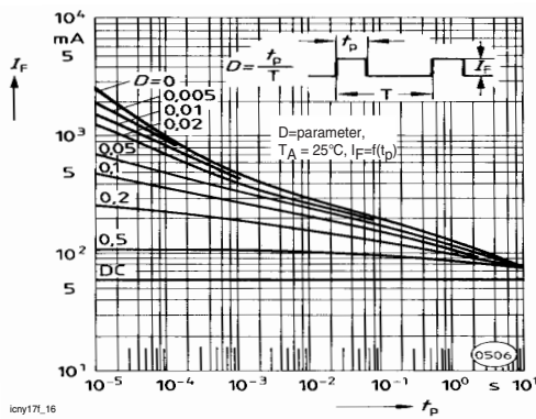
Figure 16. Permissible Pulse Load
