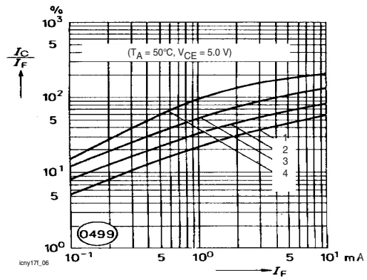
Figure 6. Current Transfer Ratio vs. Diode Current
