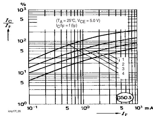
Figure 5. Current Transfer Ratio vs. Diode Current
