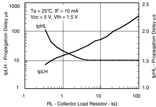
Figure 13. Propagation Delay vs. Collector Load Resistor
