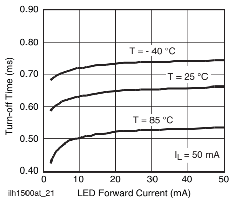
Fig. 22 - Turn-off Time vs. LED Current
