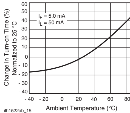
Fig. 16 - Turn-on Time vs. Temperature
