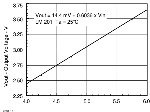
Figure 19. Transfer Gain
